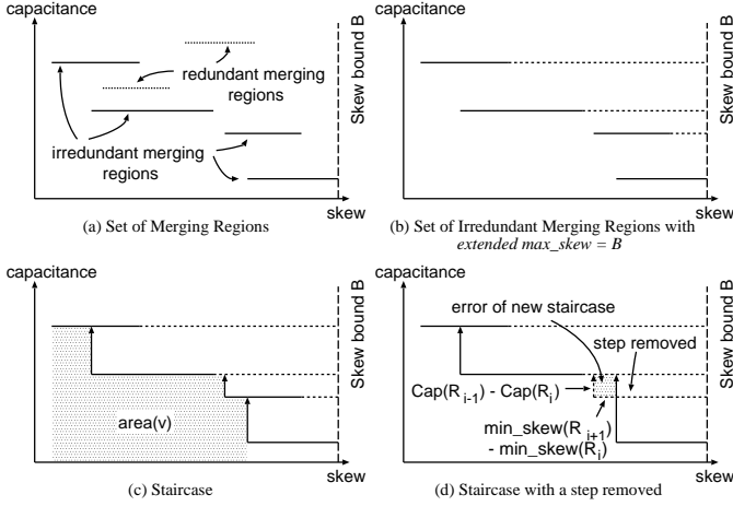
Figure 7: (a) Set of merging regions. (b) Set of irredundant merging regions with extended max_skew = B . (c) Forming a staircase from \min\_skew(R_i) to merging region R_{i-1} . (d) Removing an intermediate step results in a new staircase with an error depicted by the shaded region.
