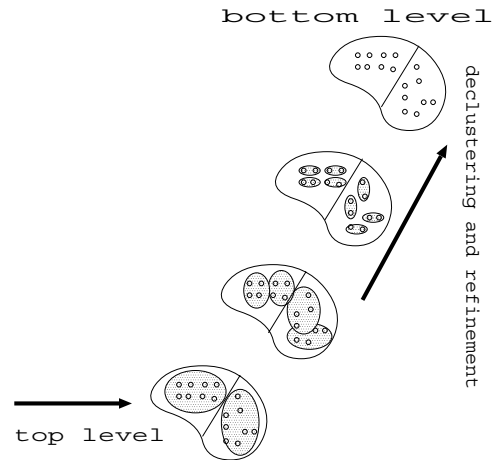
Figure 2: Top-Down Multi-Level Partitioning Method.
