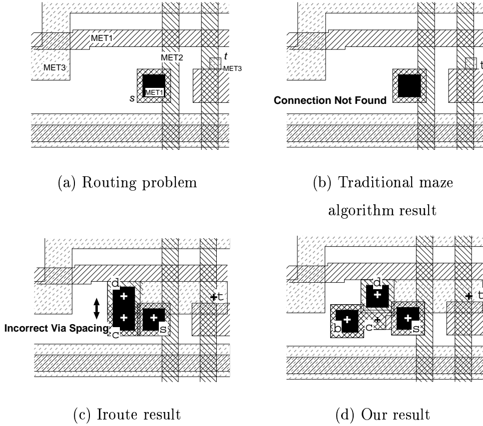
Fig. 9. A case using the 0.5\text{-}\mu\text{m} CMOS technology shown in TABLE II where our proposed routing algorithm found the via-rule correct optimal path. The starting point s is a polysilcon-to-MET1 contact and the target is somewhere to the right of the figure. The layouts are drawn to scale.
