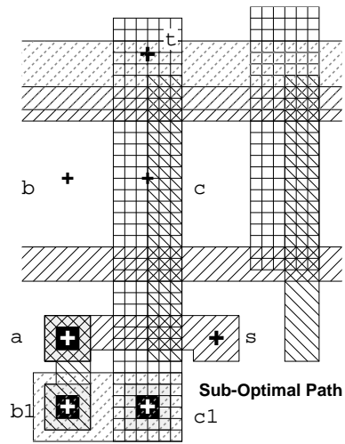
(b) Traditional maze algorithm result
