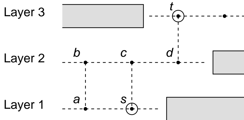
Fig. 2. An example where a traditional maze router cannot find a path from s to t due to the via spacing rule that requires a minimum via-to-via spacing of two grid-points. The valid path is s-a-b-c-d-t .
