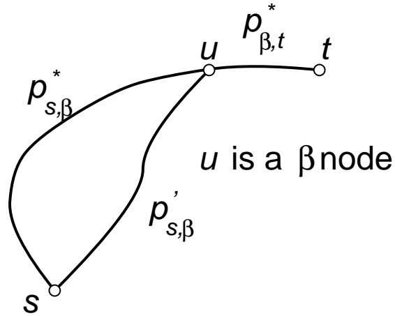
Fig. 4. Illustration of a \beta node.
