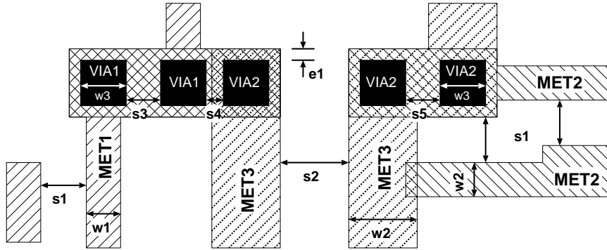
Fig. 1. Illustration of the 0.5 \mu\text{m} CMOS design rules.
