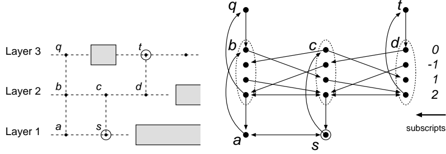
Fig. 6. The extended connection graph G' for the example shown on the left.
