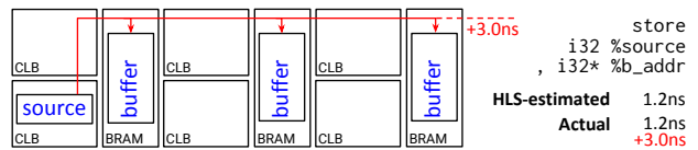
Figure 4: HLS-generated architecture of Fig. 3
