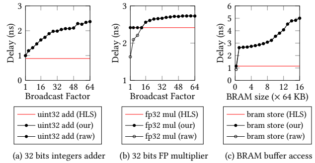
Figure 9: Vivado HLS estimated delay, our calibrated delay and raw experimental delay on different operators.
