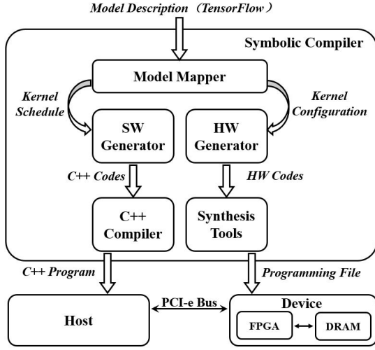
Fig. 1: FP-DNN Framework
