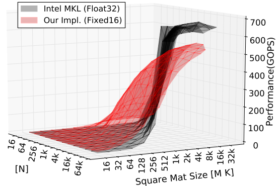
(b) Square Matrix to Rectangle Matrix Multiplication
