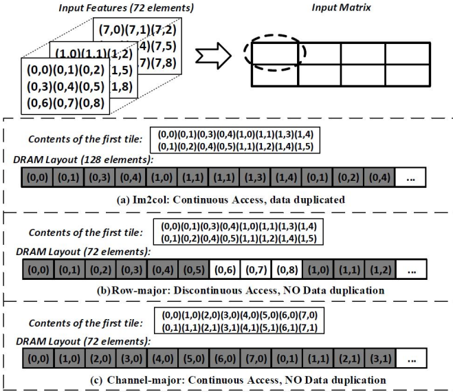
Fig. 4: Layout Optimization
